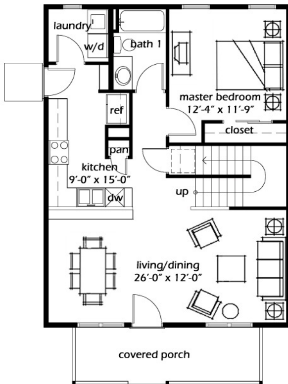
Main Level 664 sq. ft.
